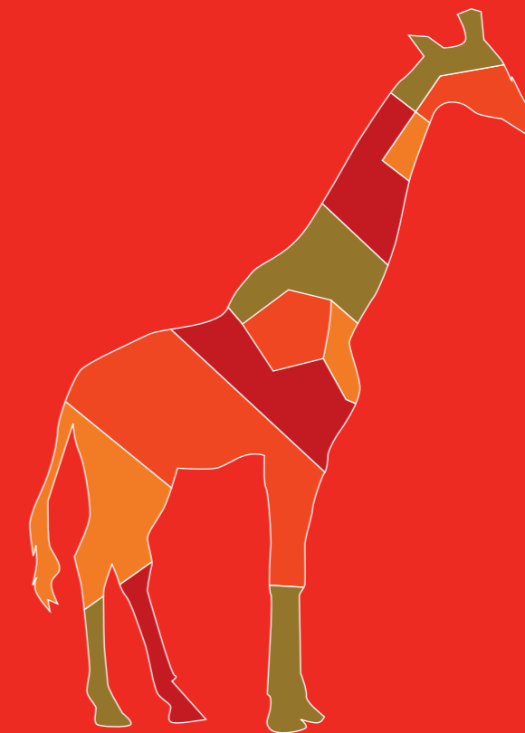
Fig. 1 ... Four-Coloring of Planar Giraffe
